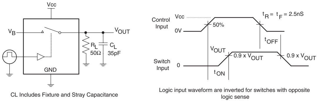
Figure 2. Turn-On/Turn-Off Timing
