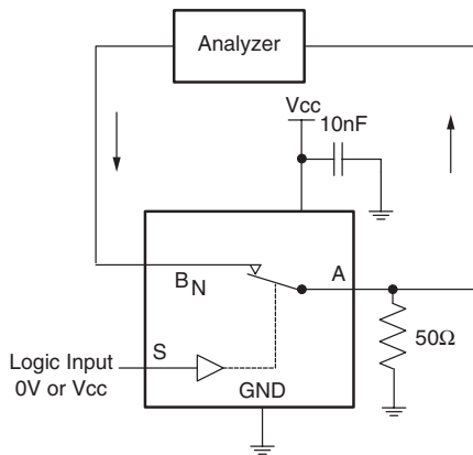
Figure 8. Bandwidth
