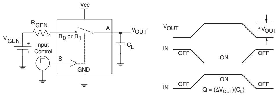
Figure 6. Charge Injection
