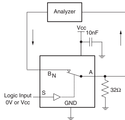
Figure 9. Harmonic Distortion
