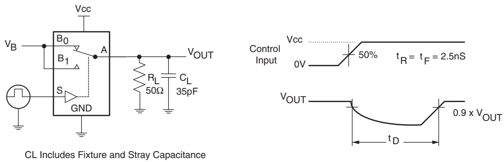
Figure 3. Break-Before-Make Timing
