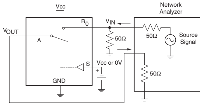
Figure 4. Off Isolation
