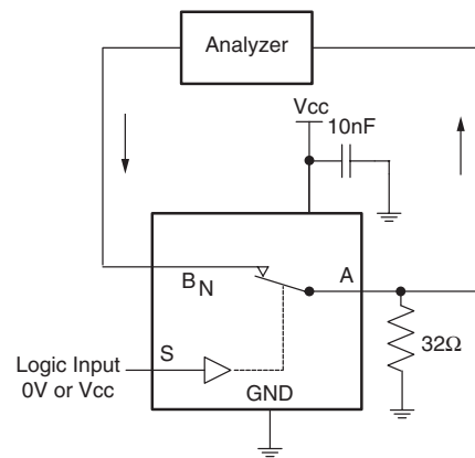
Figure 9. Harmonic Distortion
