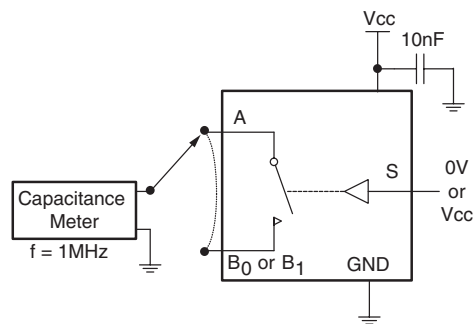
Figure 7. ON/Off Capacitance Measurement
