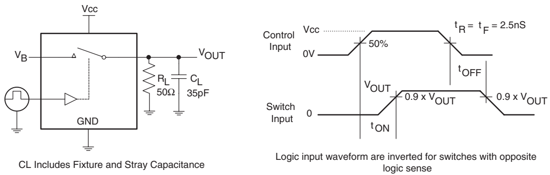
Figure 2. Turn-On/Turn-Off Timing
