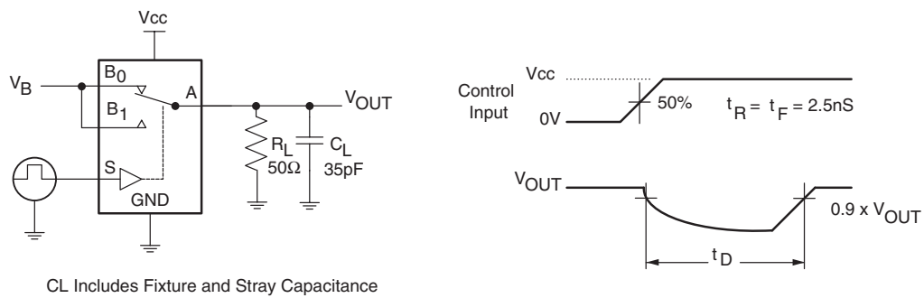
Figure 3. Break-Before-Make Timing
