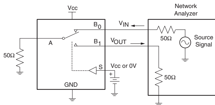
Figure 5. Crosstalk
