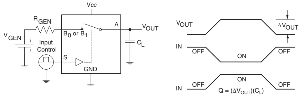
Figure 6. Charge Injection
