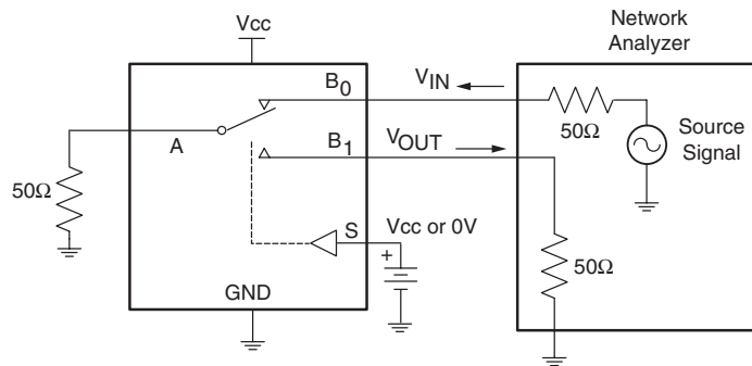
Figure 5. Crosstalk
