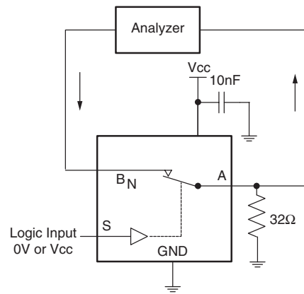
Figure 9. Harmonic Distortion
