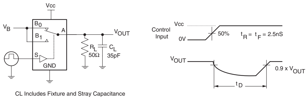
Figure 3. Break-Before-Make Timing
