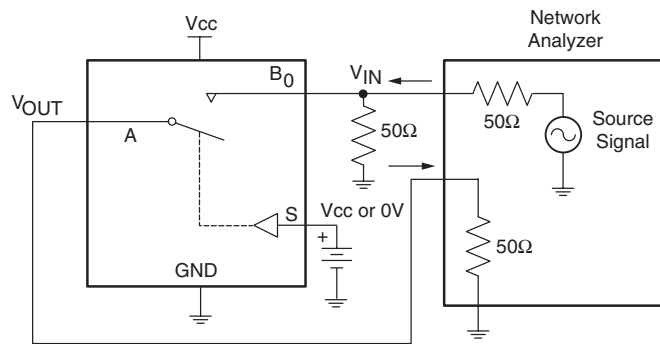
Figure 4. Off Isolation
