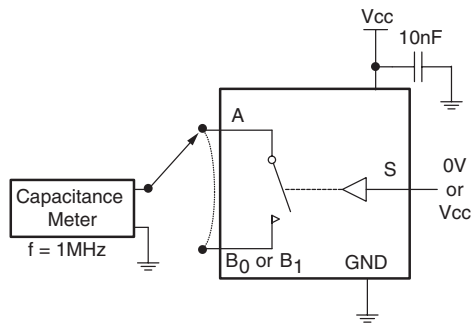
Figure 7. ON/Off Capacitance Measurement
