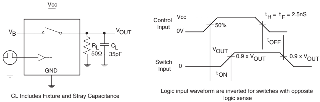
Figure 2. Turn-On/Turn-Off Timing
